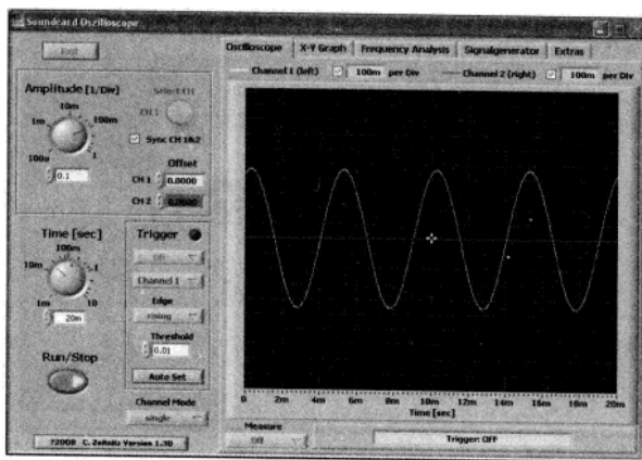
图5 Soundcard Oscilloscope
