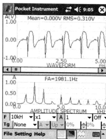
图2 Pocket Multi-Instrument
