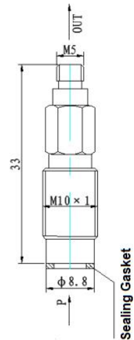
Schematic diagram
