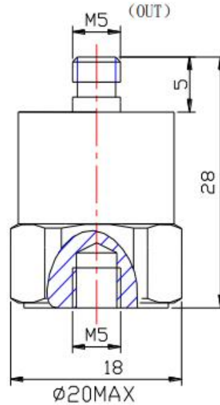
Schematic diagram
