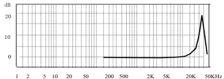
Typical Frequency Response Curve
