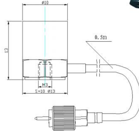
Schematic diagram
