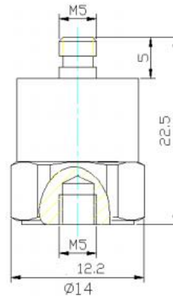
Schematic diagram
